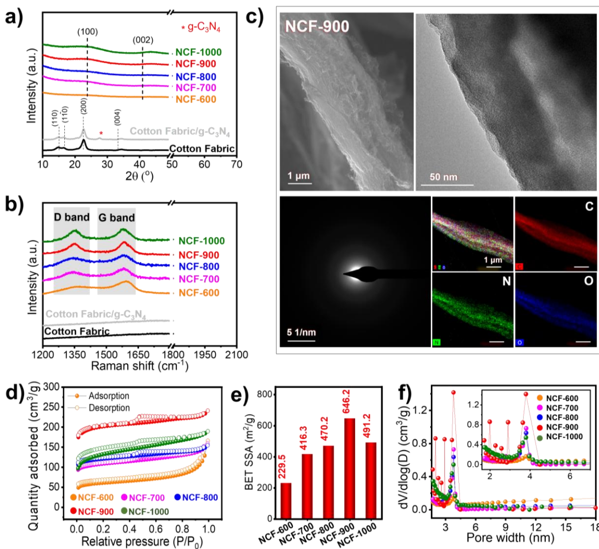
Figure 3. Structural and morphological characterization of cotton fabric, cotton/g-C 3 N 4 precursor, and NCF-T samples (T = 600–1000 ^\circ C). a) XRD patterns showing the gradual evolution from amorphous carbon to partially graphitized domains with increasing pyrolysis temperature; b) Raman spectra displaying D and G bands, where the highest I D /I G ratio in NCF-900 indicates the highest defect density associated with nitrogen incorporation; c) SEM, TEM, and SAED images of NCF-900 revealing a porous and partially ordered carbon framework. TEM–EDS (energy dispersive x-ray spectroscopy) elemental mapping confirms the presence of C, N, and O distribution within the carbon framework; d) Nitrogen adsorption–desorption isotherms of NCF-T samples showing type IV behavior with distinct hysteresis loops characteristic of mesoporous structures; e) BET-specific surface areas of NCF-T samples, revealing the maximum surface area of \sim 646 m 2 g -1 for NCF-900 compared to other temperatures, which supports its superior electrochemical performance. f) BJH (Barrett, Joyner, Helenda) pore-size distributions confirming mesopores centered at \sim 3.9 nm for NCF-900, favorable for electrolyte ion transport. Cumulative pore-volume plots indicate the highest total pore volume for NCF-900, consistent with its enhanced mesoporosity and ion accessibility.
